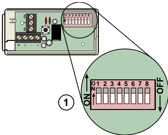
1 - Address switches
