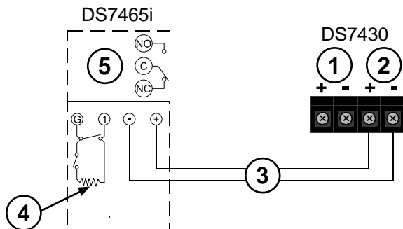
Figure 3: DS7430 Multiplex Expansion Module Wiring
